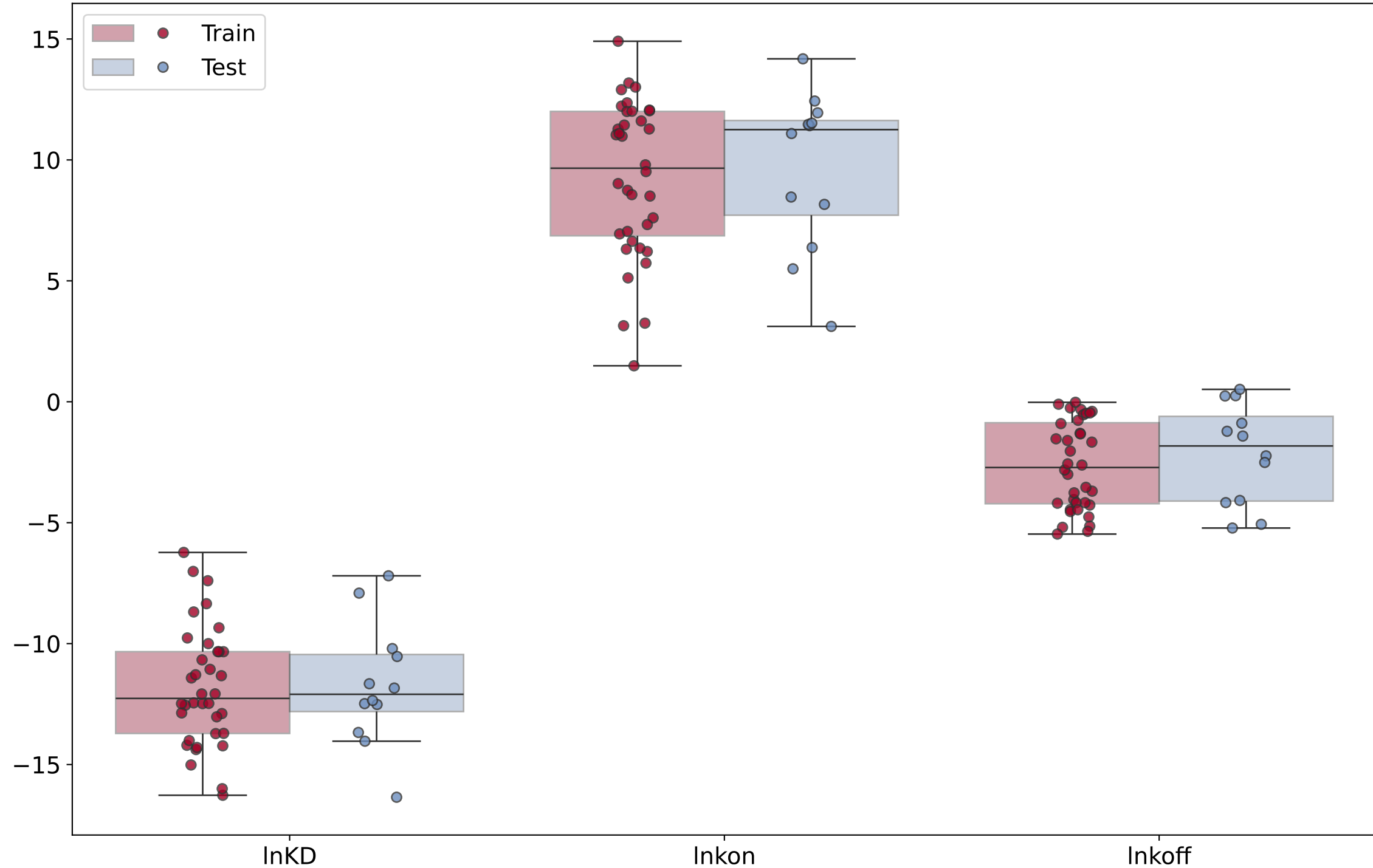
Distribution of Target Variables in Train and Test Sets
