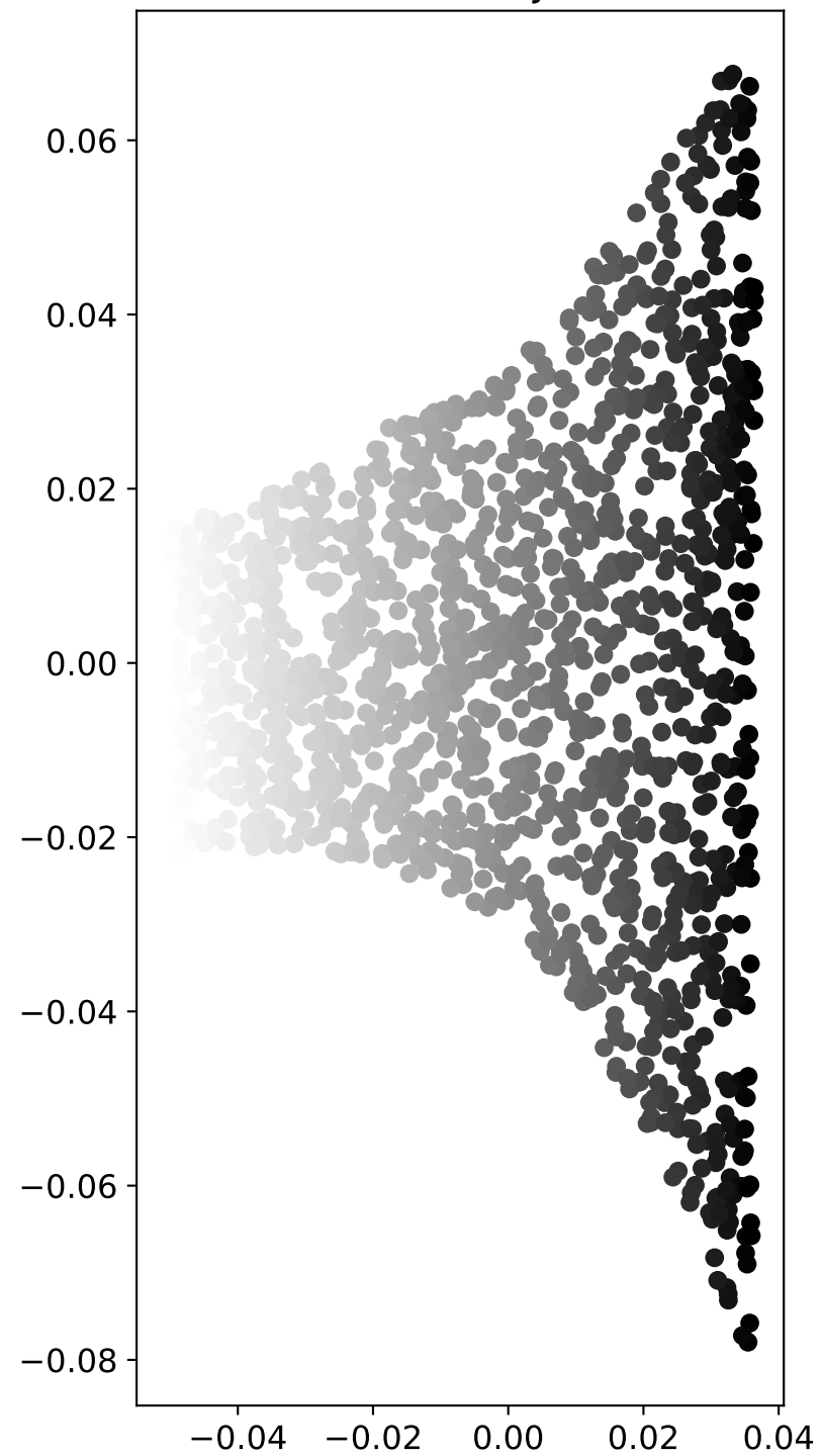
Nonlinear Projection
