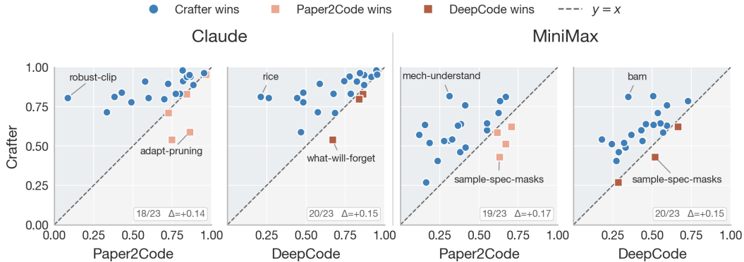
Figure 2: Per-paper Code-Dev: Crafter vs. each baseline. Each panel pairs one backend (Claude / MiniMax) with one baseline (Paper2Code / DeepCode). A point is one paper at coordinates (baseline, Crafter). Points above the y = x diagonal (blue circles) are papers where Crafter outperforms the baseline; points below (orange / red squares) are papers where the baseline wins. The papers with the largest gain and the largest loss (by \Delta = \text{Crafter} - \text{baseline} ) are annotated in each panel; corner boxes report wins / 23 and the mean \Delta .
