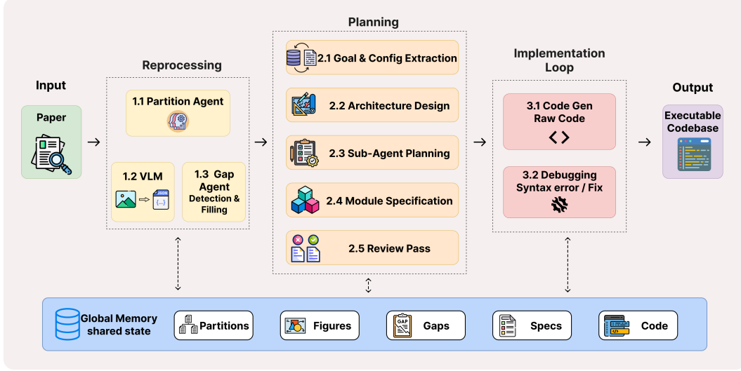
Figure 1: Crafter architecture. Ten types of agent across 3 stages pass information through a shared GlobalMemory. The partition agent decomposes the paper into structured partitions, which feed the VLM and gap analysis. Preprocessing outputs are passed to the planning agents, which produce the implementation plan used by the implementation loop.
