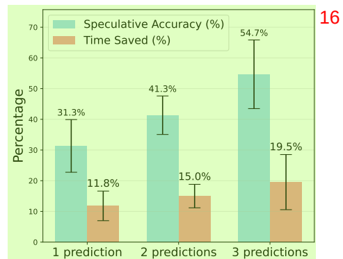
Figure 2: Percentage of time saved and percentage of correct predictions across 5 runs at 30 steps.
