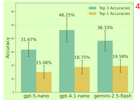
4 Figure 4: Accuracy with gemini-2.5-flash as the Actor. Speculating multiple actions ( k = 3 ) yields higher accuracy than predicting a single action.
