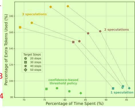
Figure 6: Cost-latency tradeoff across different speculation widths, forming a Pareto curve. 7
