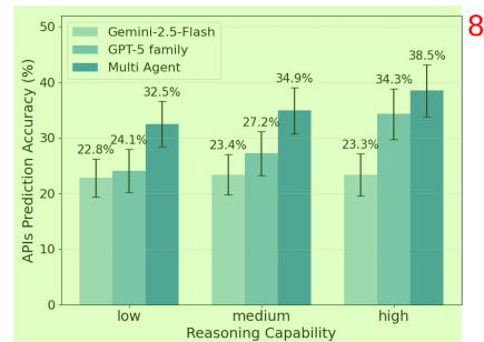
Figure 3: APIs prediction accuracy across various Speculator models. 9
