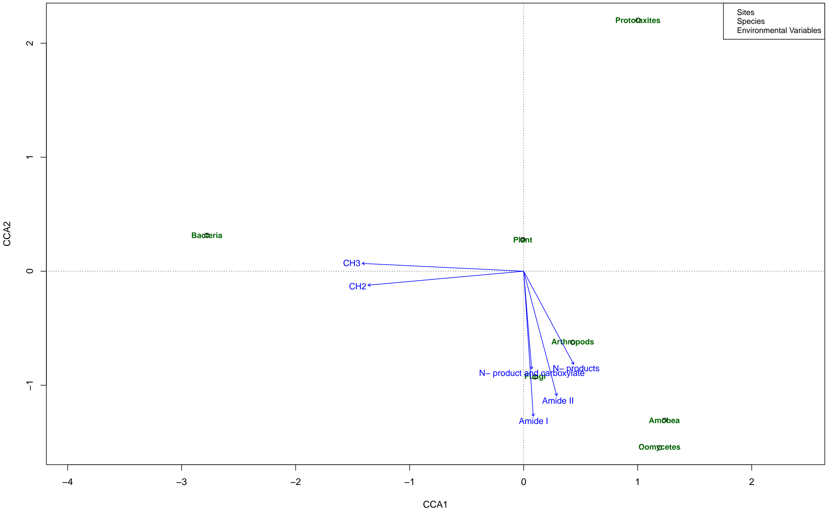
CCA Biplot
