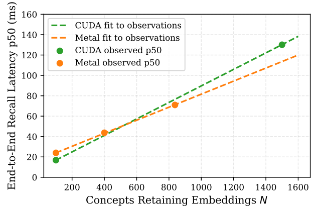
Figure 4: End-to-end recall p50 observations from Issue 8 and linear fits. Each CUDA size has 12 timed recalls after two warmups. Each Metal size has 24 timed recalls after two warmups. Dashed lines extend the fitted models beyond the measured sizes.
