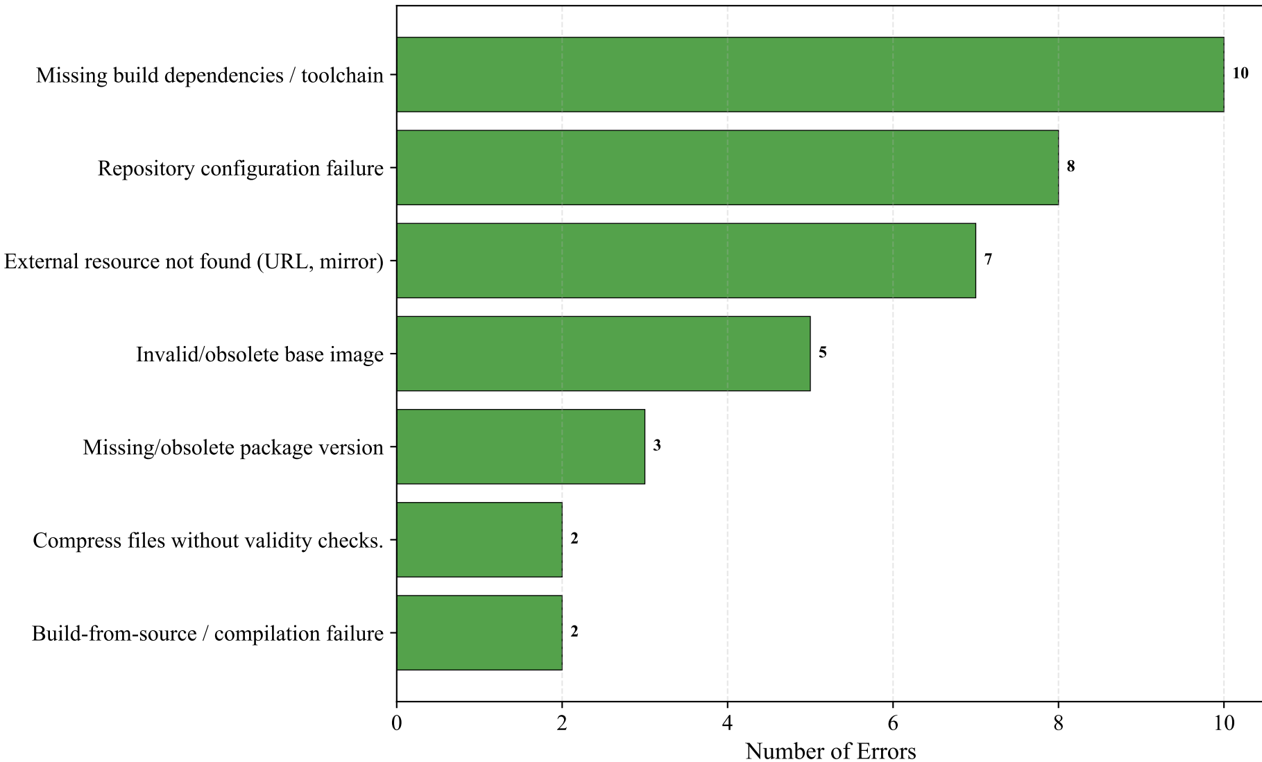
Build Error Category
