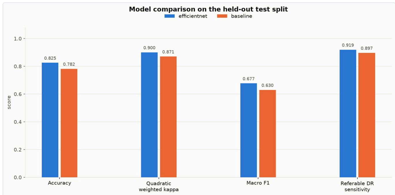
Model comparison on the held-out test split.
