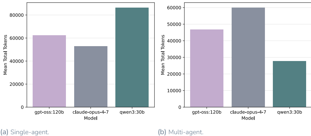
Figure 6.2.: Mean total token usage per model (Containerlab, n = 10 runs each).
