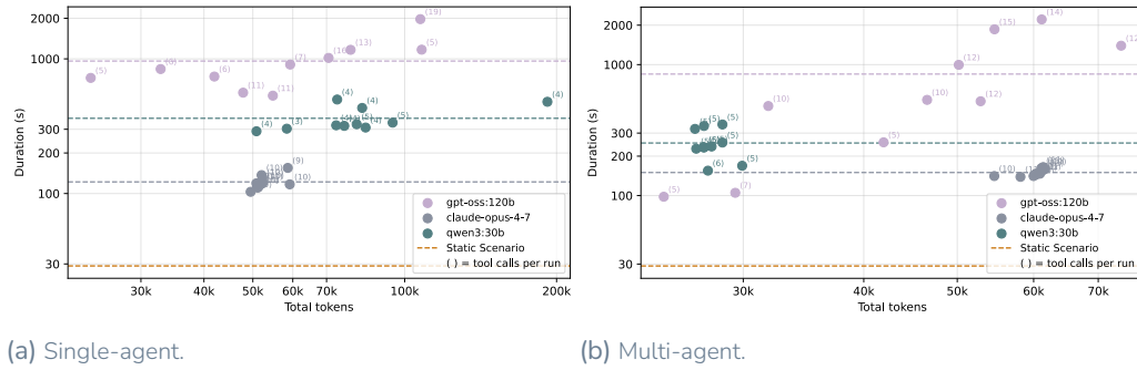
Figure 6.3.: Total tokens vs. run duration per individual run (Containerlab, n = 10 per model).
