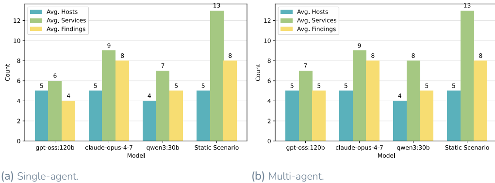
Figure 6.4.: Average hosts, services, and findings discovered per model (Containerlab, n = 10 runs each).
