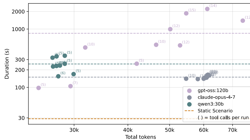
Figure 6.3.: Total tokens vs. run duration per individual run (Containerlab, multi-agent, n = 10 per model).
