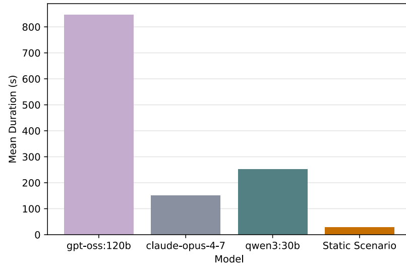
Figure 6.1.: Mean run duration per model (Containerlab, multi-agent, n = 10 runs each).
