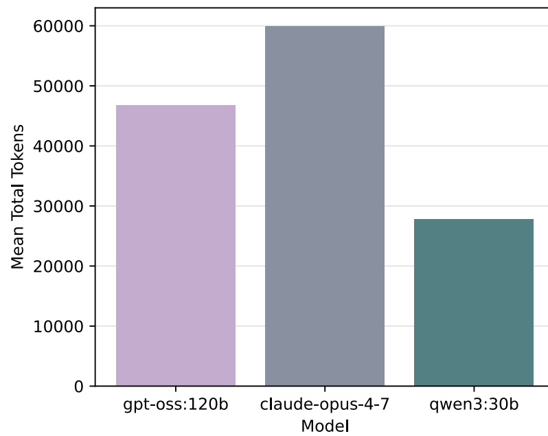
Figure 6.2.: Mean total token usage per model (Containerlab, multi-agent, n = 10 runs each).
