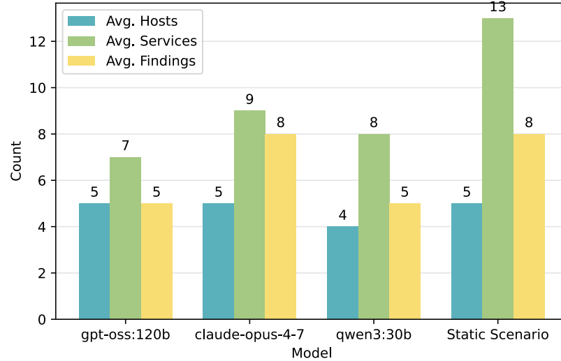
Figure 6.4.: Average hosts, services, and findings discovered per model (Containerlab, multi-agent, n = 10 runs each).
