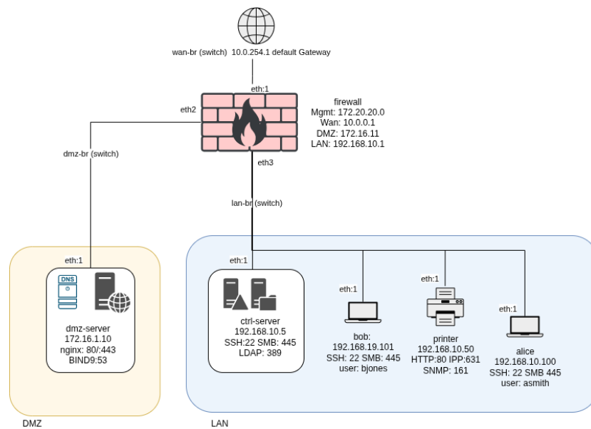
Figure 5.2.: topology-test-environment
