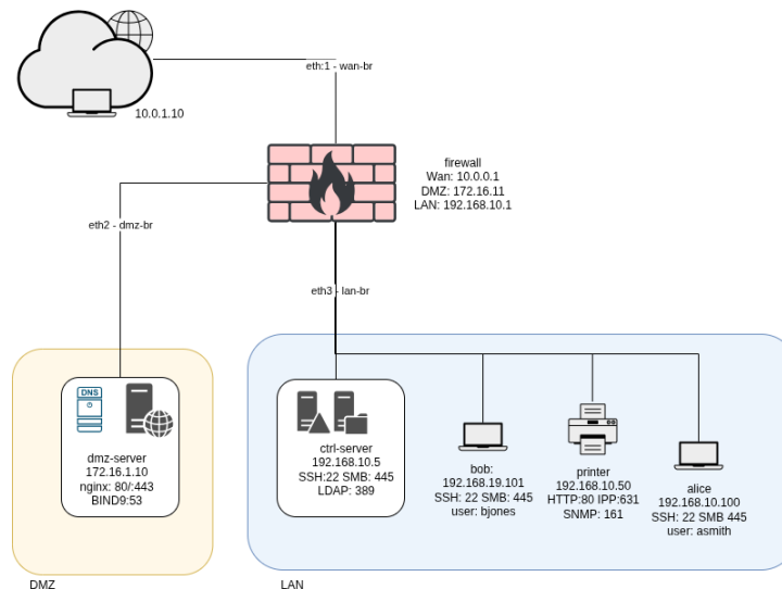
Figure 5.2.: topology-test-environment
