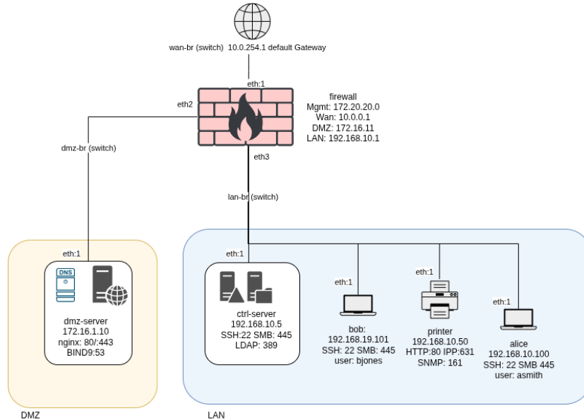
Figure 5.2.: topology-test-environment
