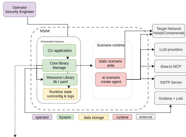
Figure 3.2.: Container view of the NSAK framework (C4 level 2).
