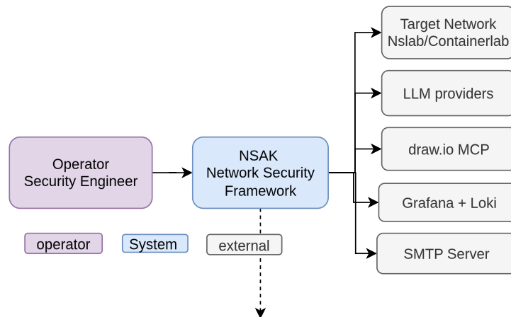
Figure 3.1.: System context of the NSAK framework (C4 level 1).
