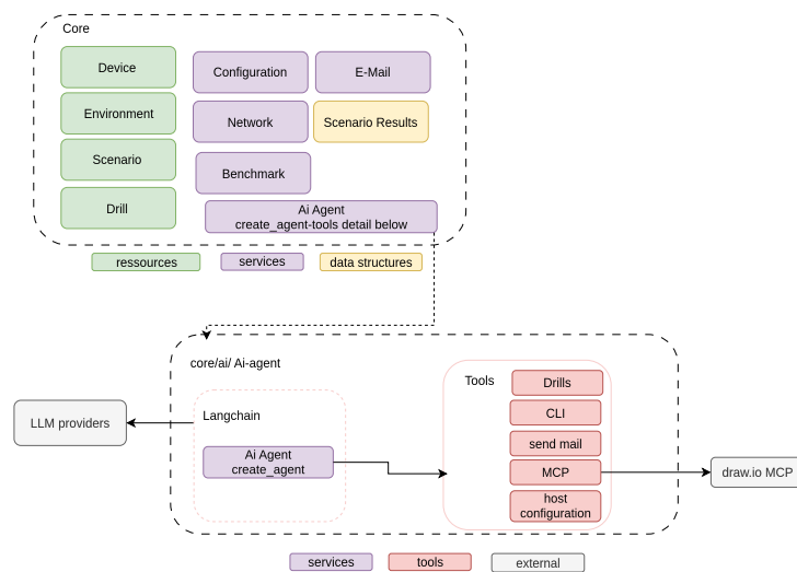
Figure 3.3.: Component view of the NSAK core (C4 level 3).
