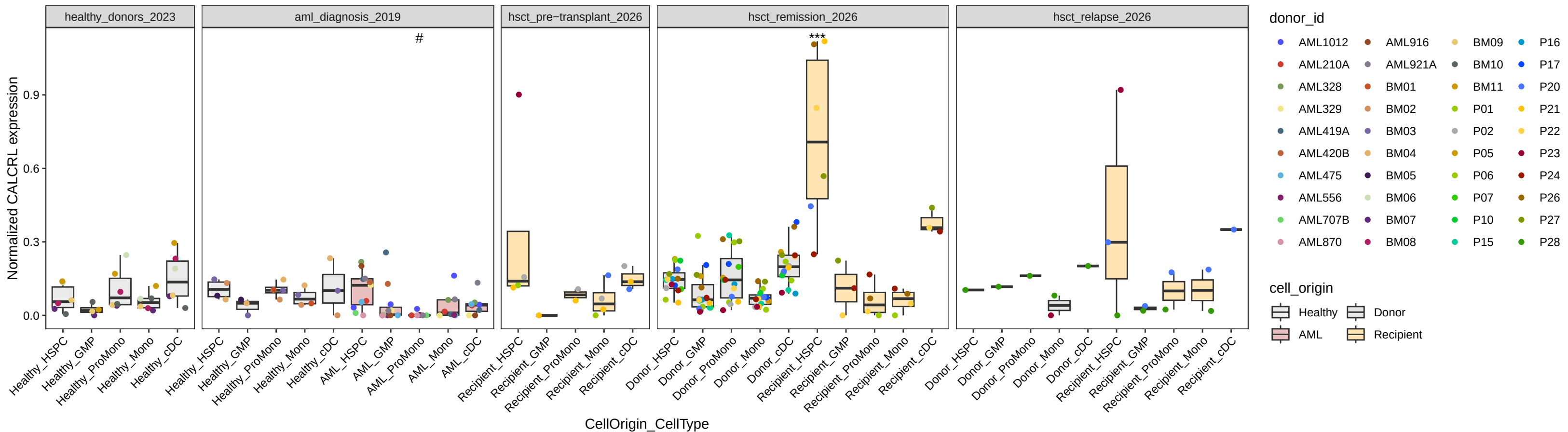
CALCRL expression across three studies
