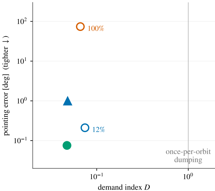
(a) Boresight pointing
