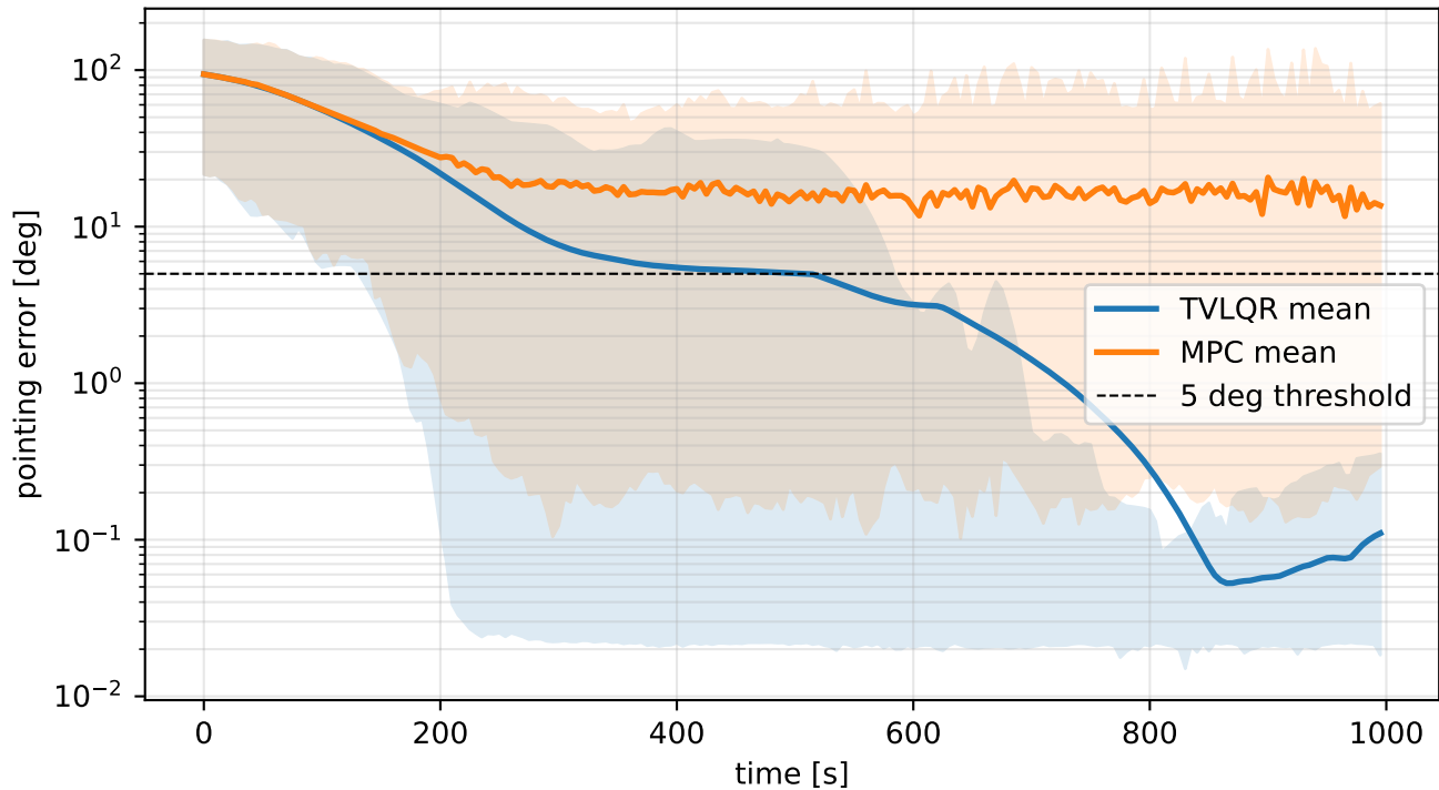
P2.4: TVLQR vs single-step MPC tracking
