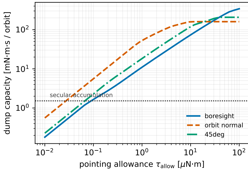
Per-orbit dump capacity
