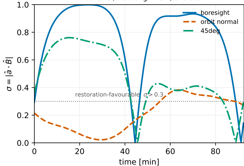
Wheel-axis / field alignment, one orbit
