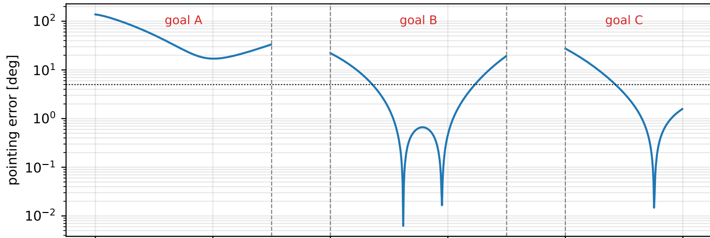
P2.3 multi-goal, 3+1 (trial 0)
