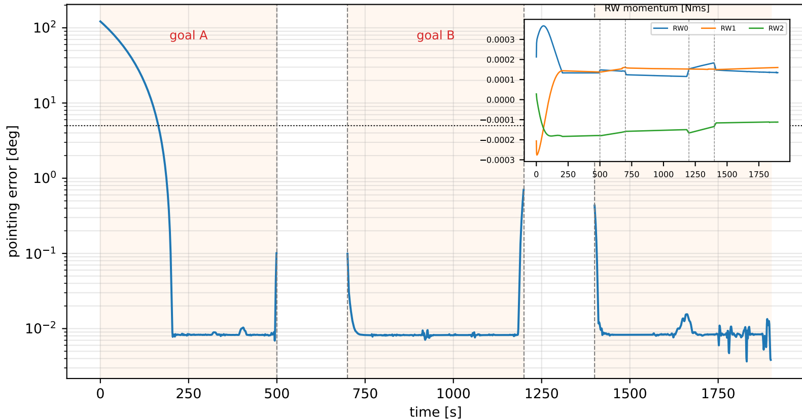
P2.3 multi-goal, 3+3 (trial 16, active=500s coast=200s)
