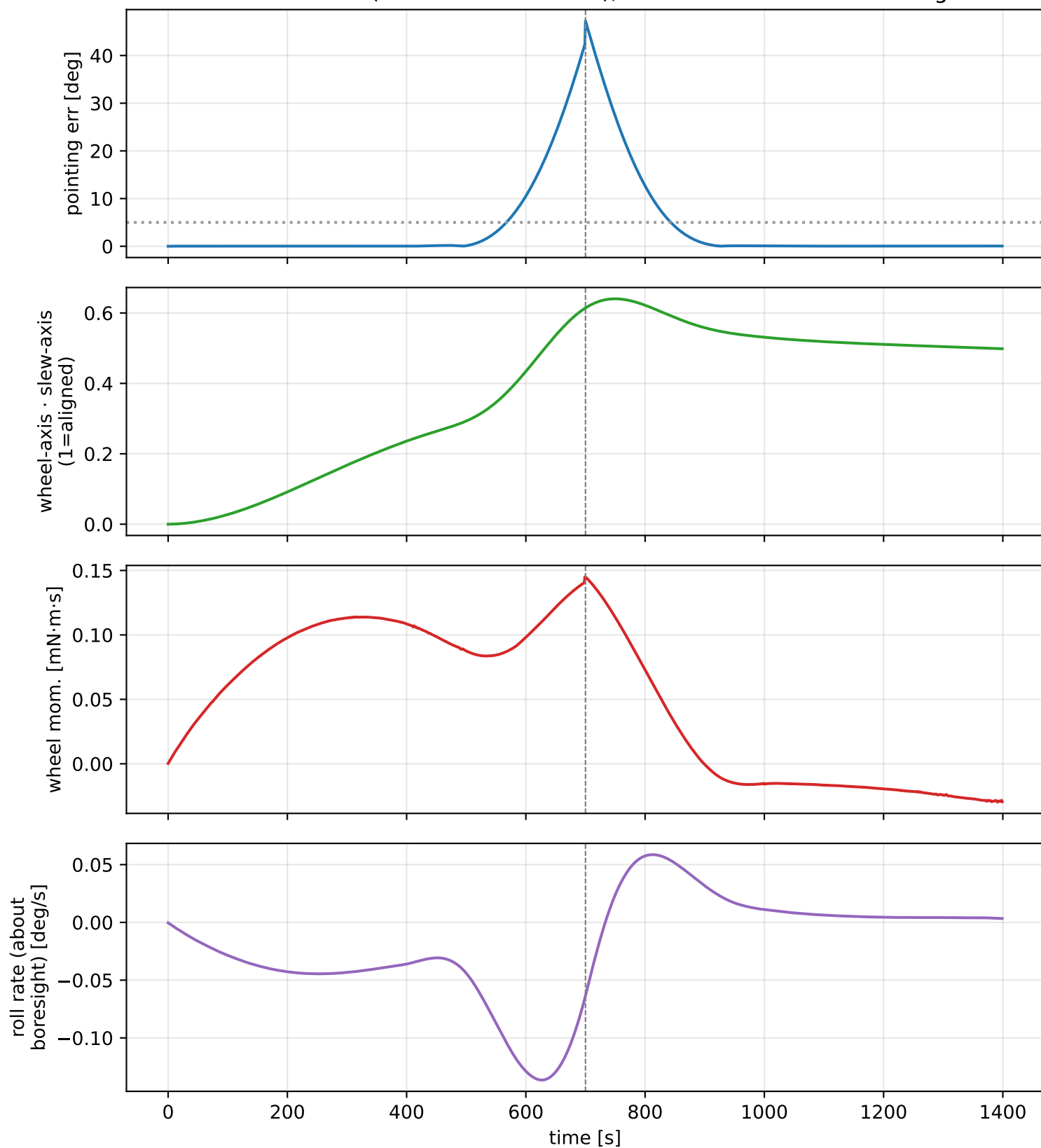
3+1 vector A→B (90° slew at t=700 s); roll free under the reduced goal.
