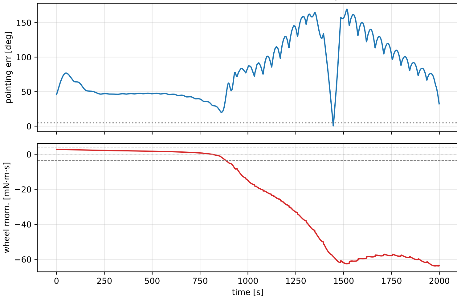
C2: disturbance-assisted desat (modeled 0.2 A·m 2 dipole, 3+1 vector)
