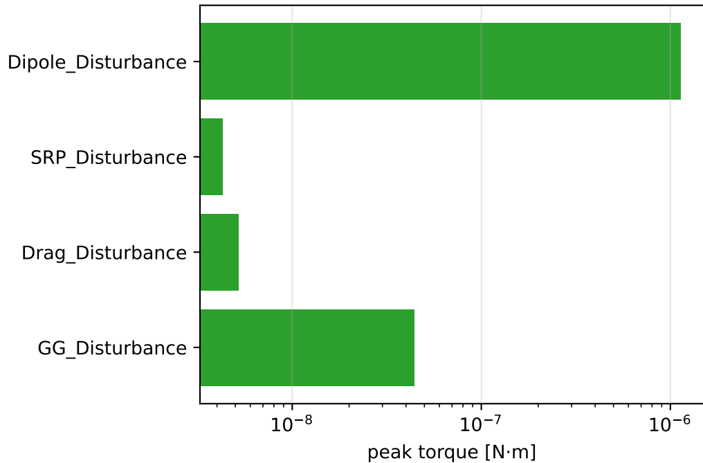
Realized plant disturbances
