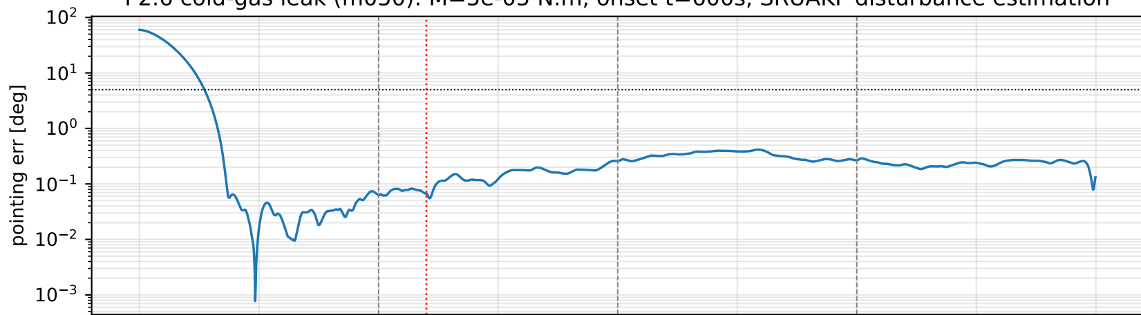
P2.6 cold-gas leak (m050): M=5e-05 N.m, onset t=600 s, SRUAKF disturbance estimation
