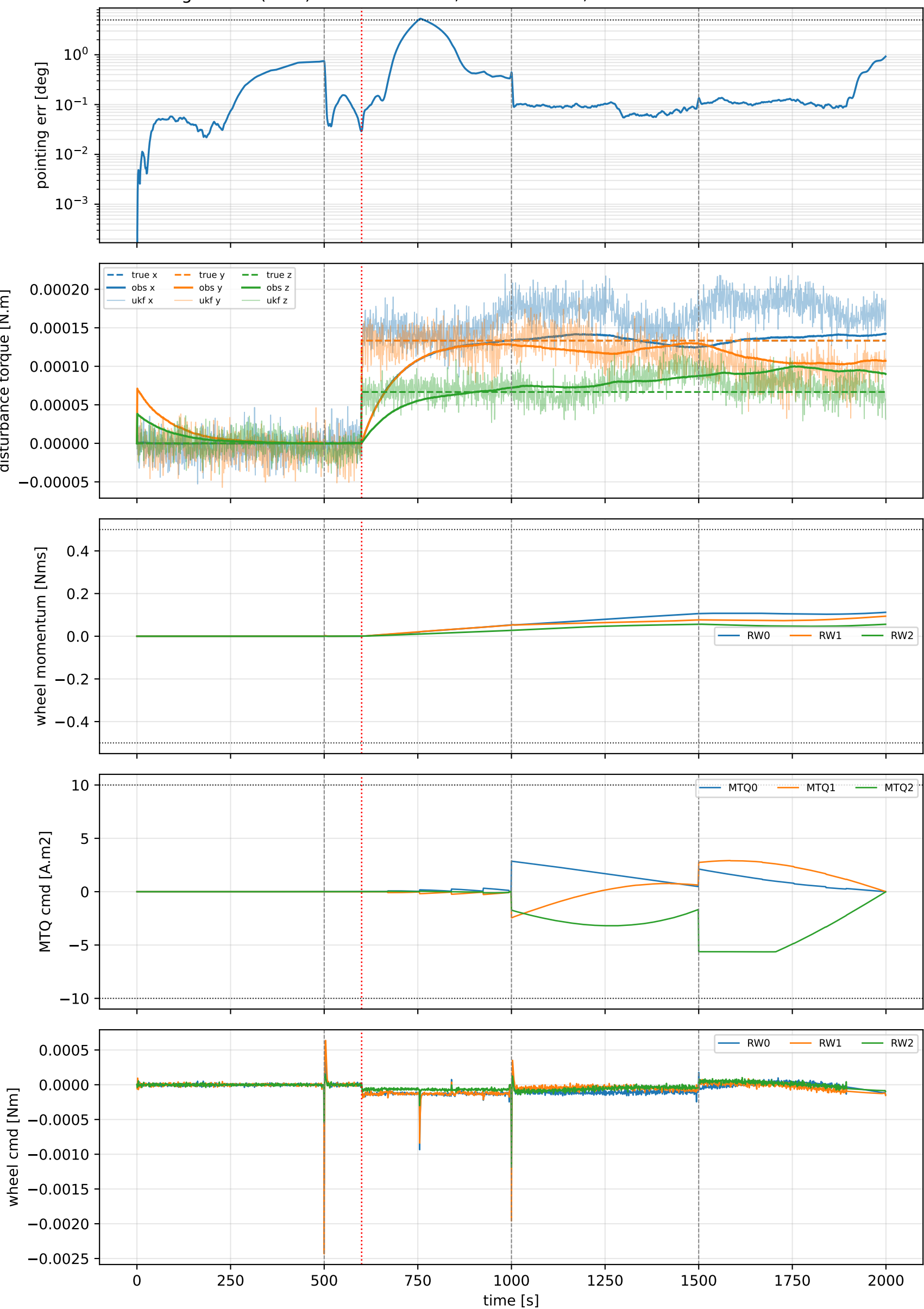
P2.6 cold-gas leak (med): M=0.0002 N.m, onset t=600 s, momentum-rate disturbance observer
