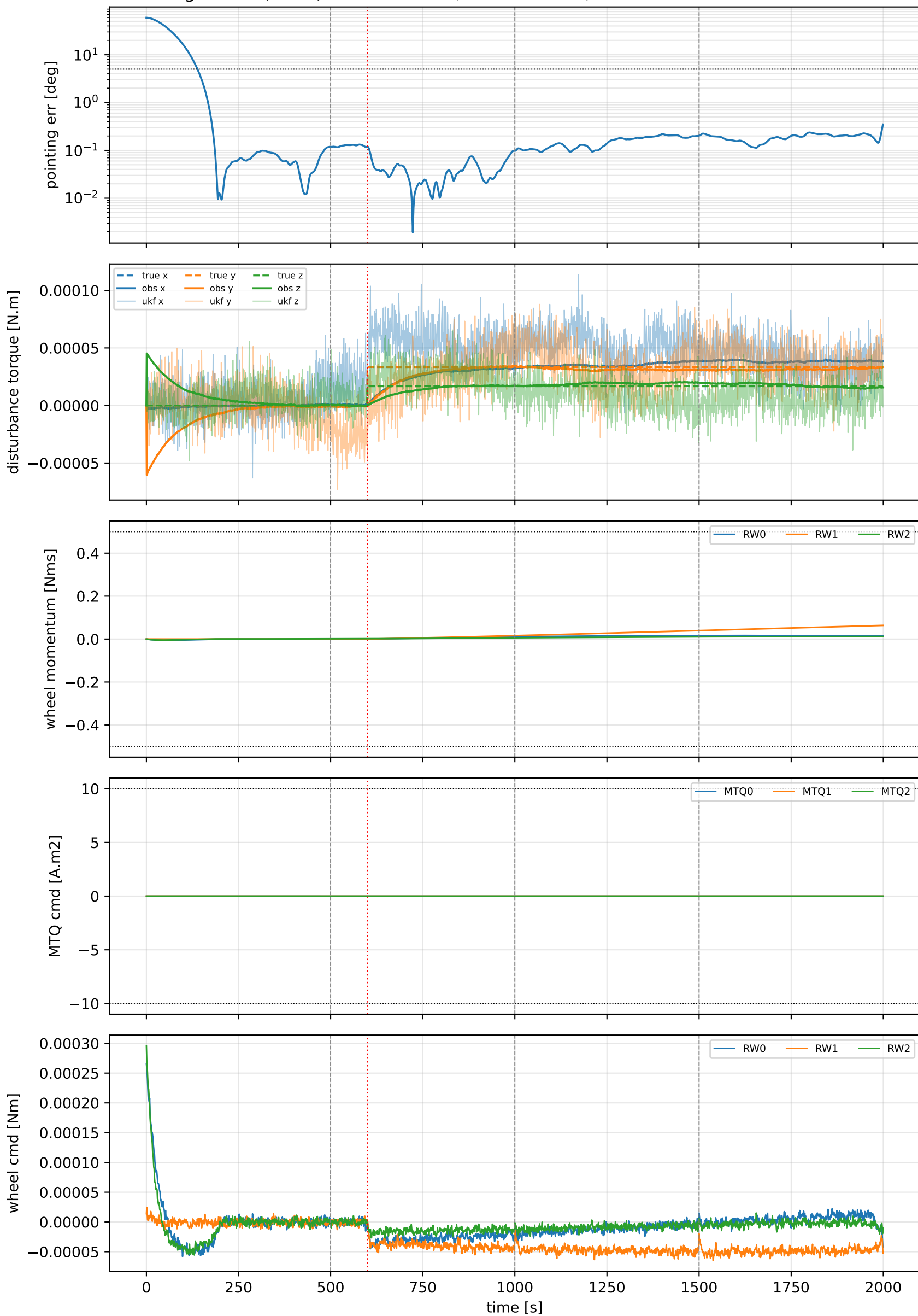
P2.6 cold-gas leak (small): M=5e-05 N.m, onset t=600 s, momentum-rate disturbance observer
