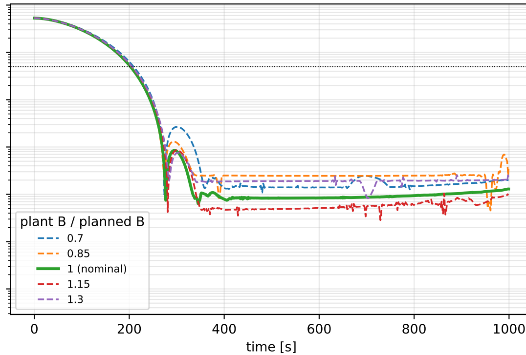
B-field magnitude mismatch
