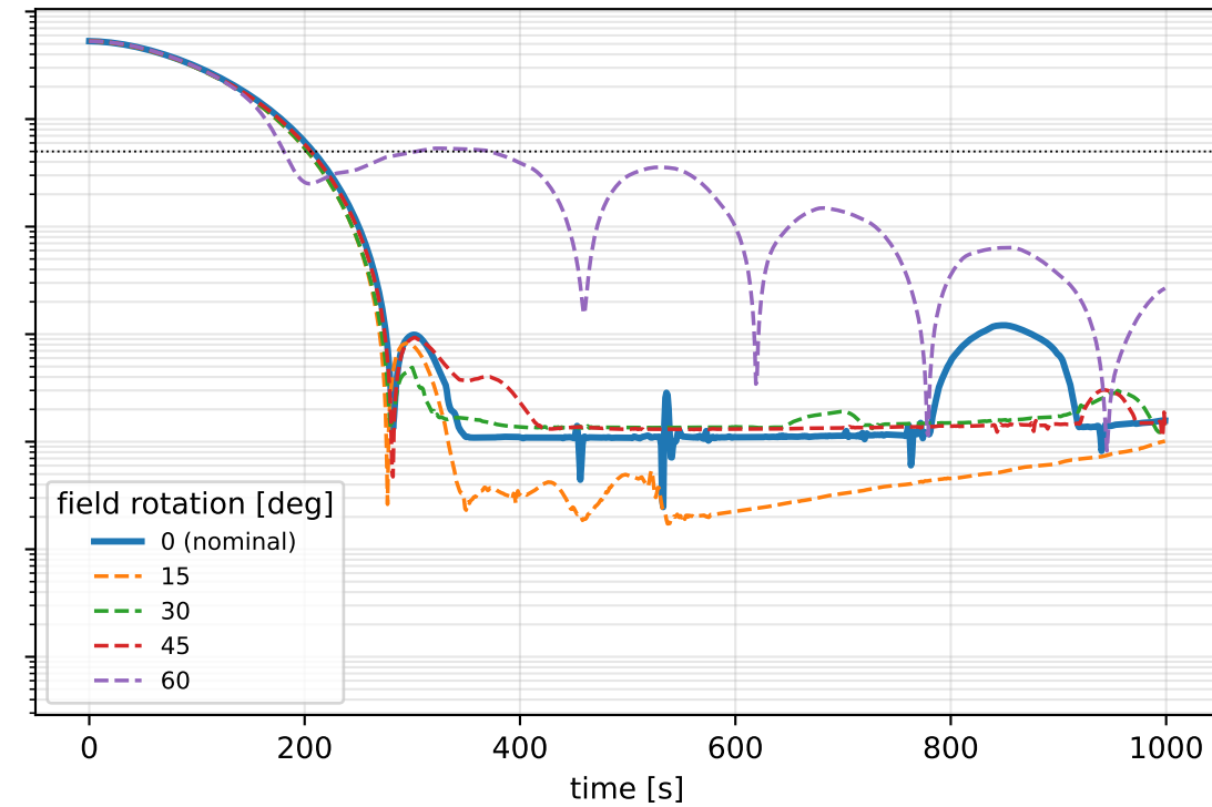
B-field rotation mismatch
