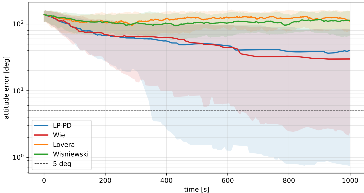
P1.3 (FIG-DIFFLAW-MC): four laws, 3MTQ+1RW, full-attitude, n=100
