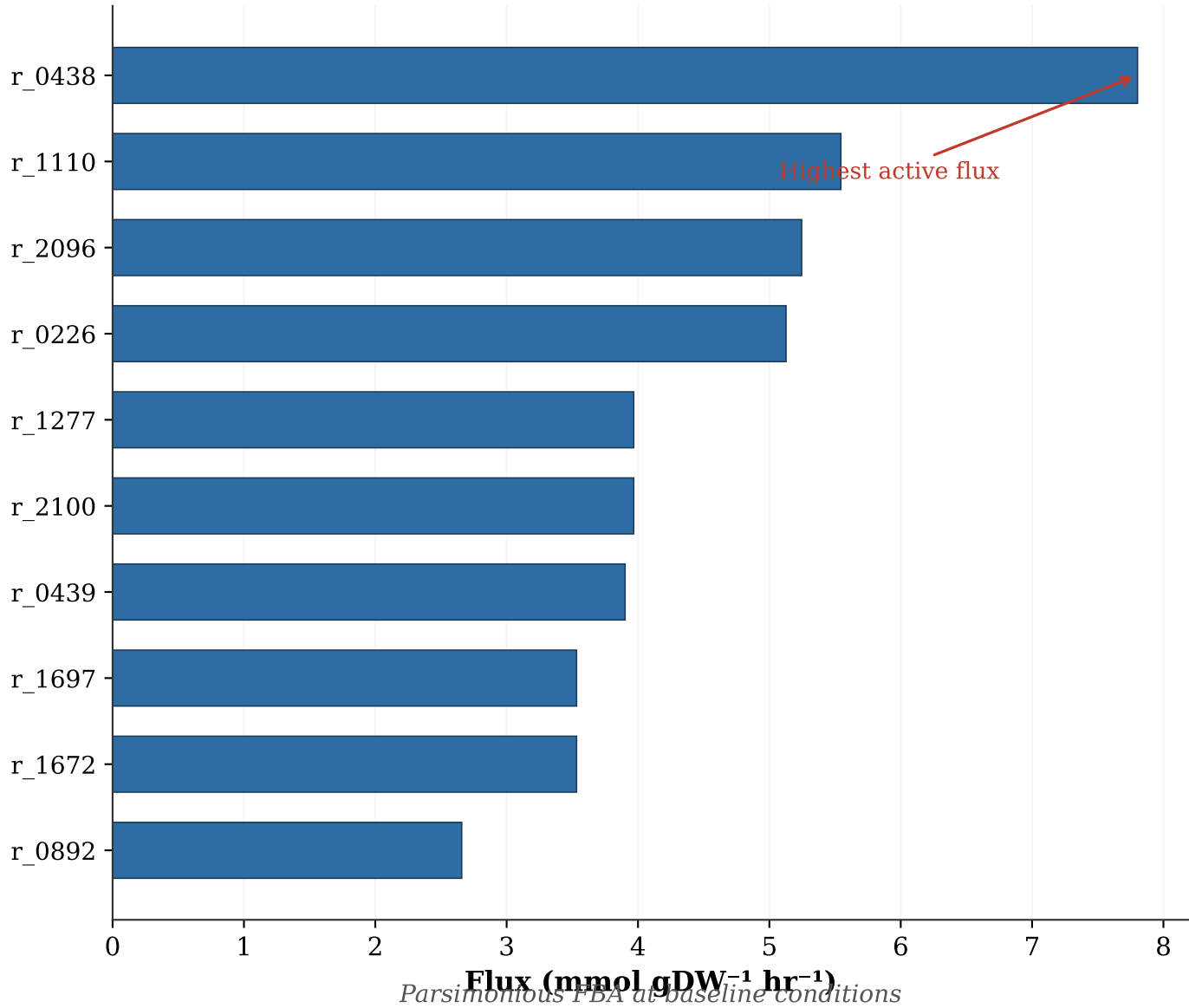
B Top 10 Active Reactions (pFBA)
