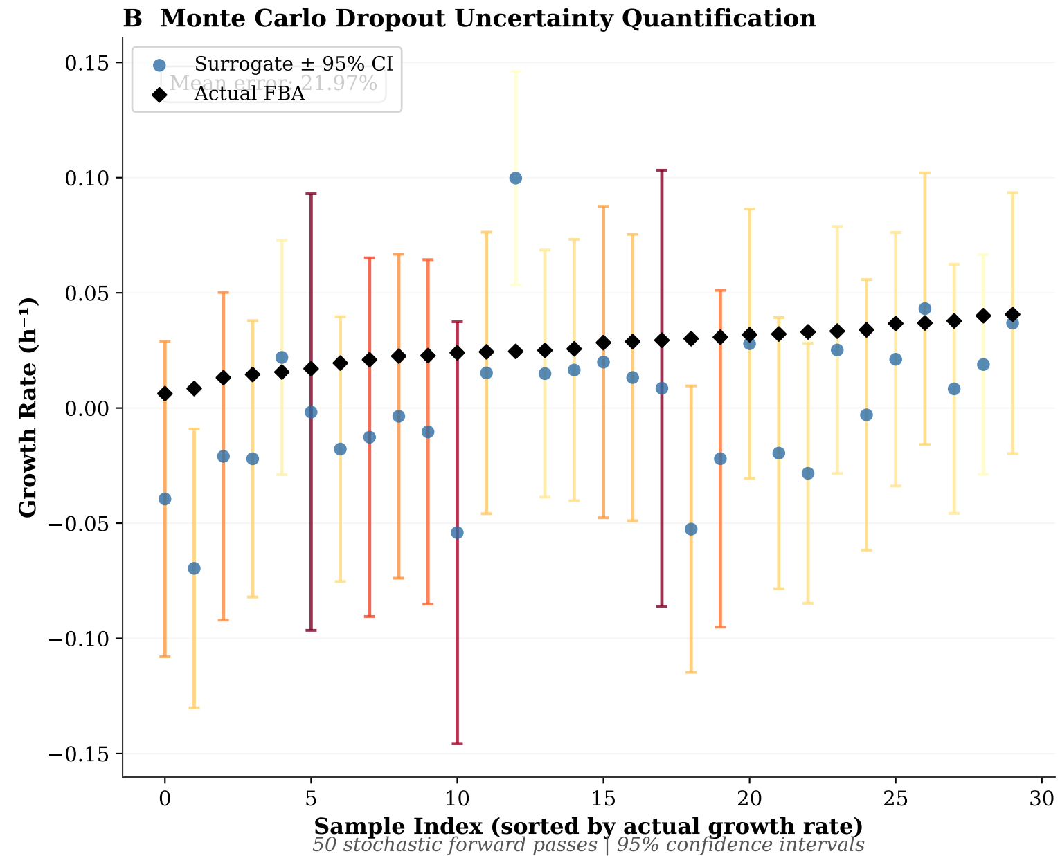
Figure 5. CNN Surrogate Model Validation and Uncertainty Quantification
