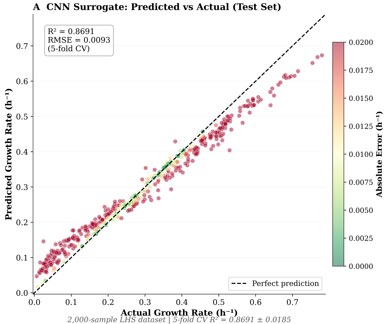
Figure 5. CNN Surrogate Model Validation and Uncertainty Quantification
