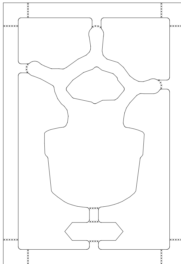
Drill Map: × 0.500mm / 0.0197" (72 holes) (not plated)
