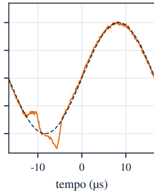
(c) subtrator, 30 kHz
