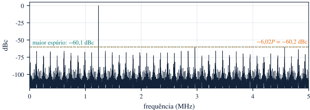
(a) amostras do DDS: f_{out} = 1,235 \text{ MHz} , N = 32 , P = 10 , D = 8
