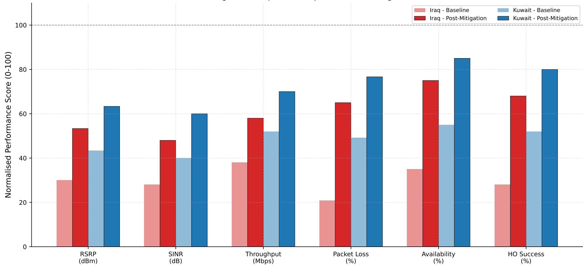
Figure 10 - Mitigation Impact on Network KPIs at 45 °C Enhanced cooling, resilient power, adaptive beamforming and 8T8R MIMO
