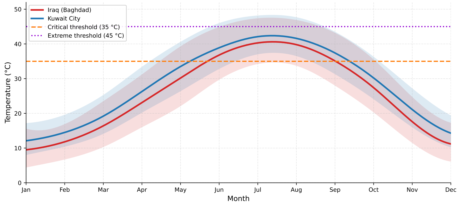
Figure 1 - Mean Monthly Temperature Profiles: Iraq vs Kuwait 2015-2023 measurement-location averages
