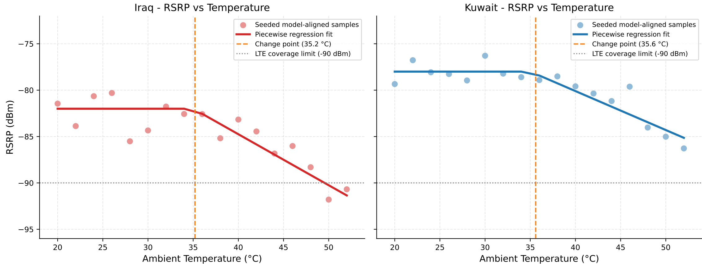
Figure 2 - Ambient Temperature Effect on RSRP
