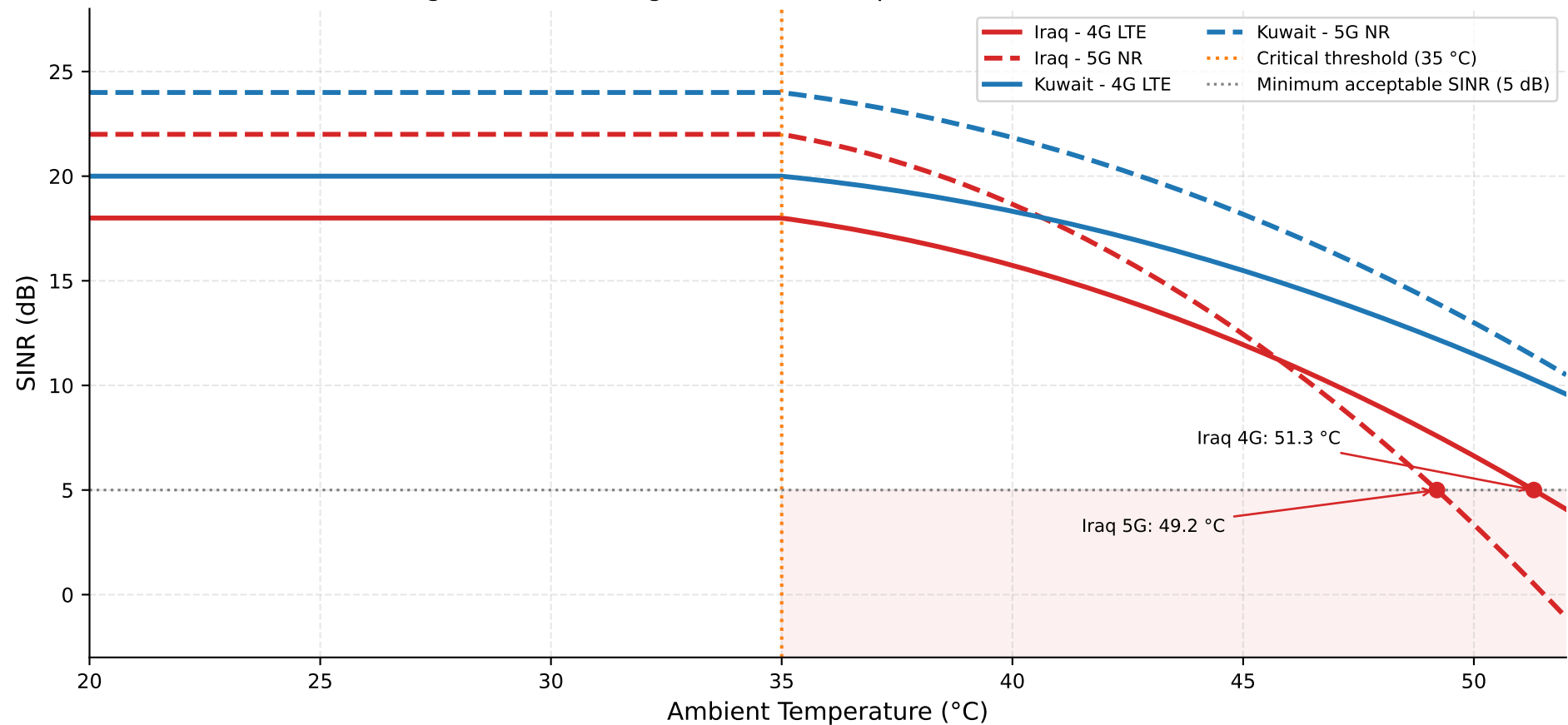
Figure 3 - SINR Degradation vs Temperature: 4G LTE and 5G NR
