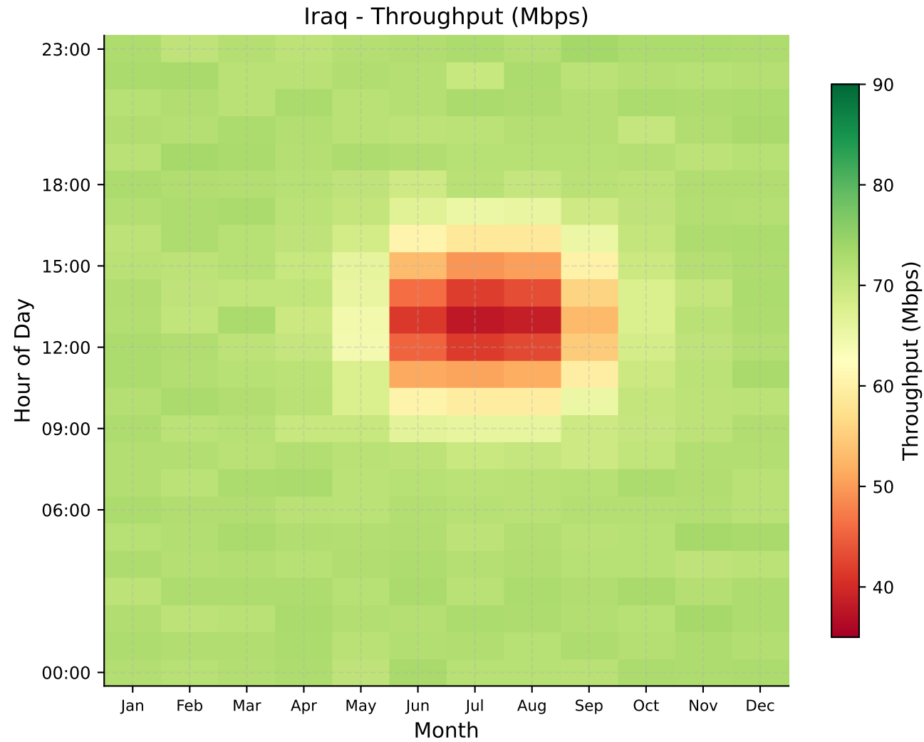
Figure 5 - Average Downlink Throughput by Hour and Month
