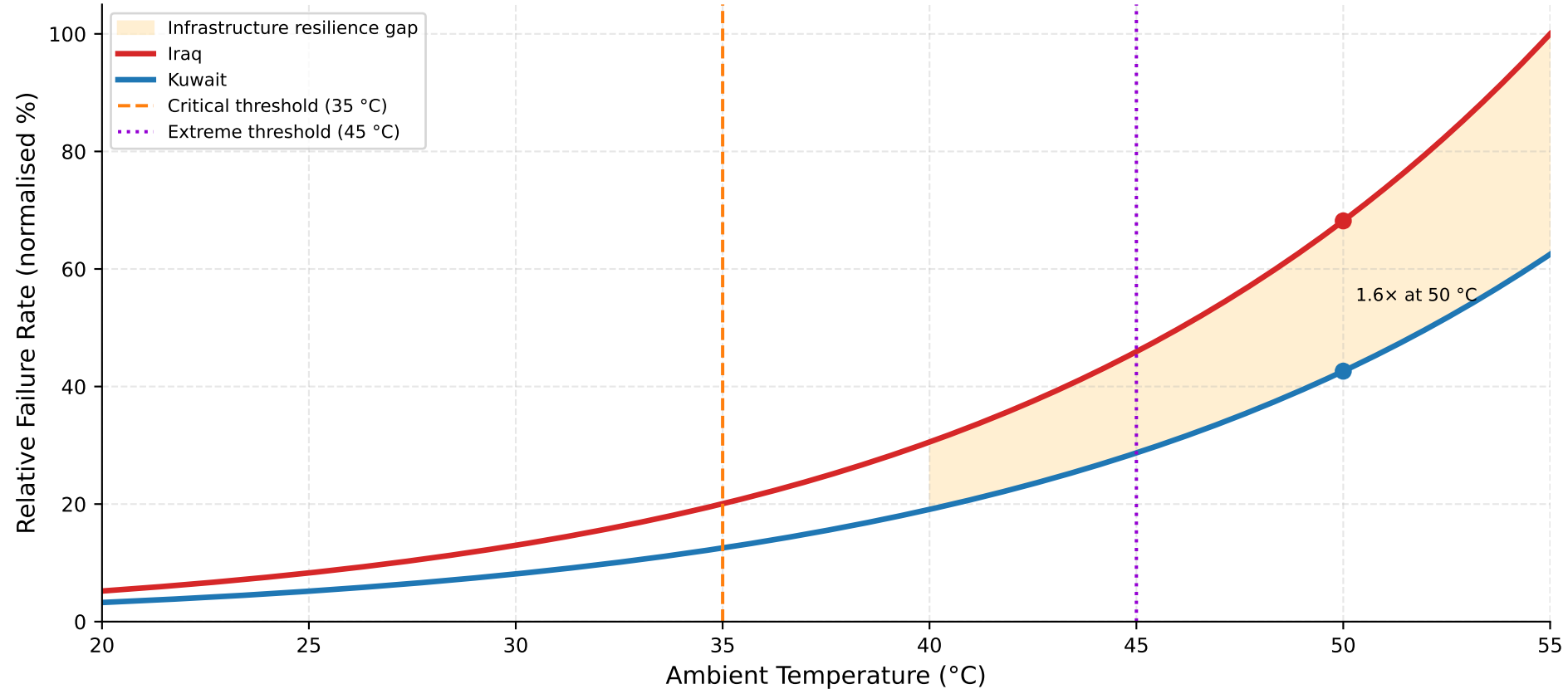
Figure 6 - Base Station Failure Rate vs Temperature Arrhenius model with E_a = 0.7 eV
