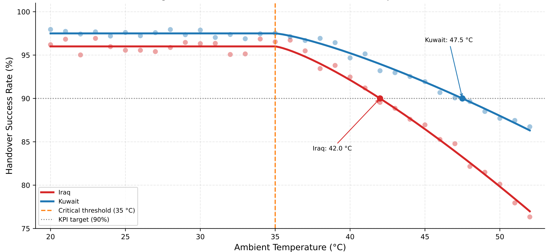
Figure 8 - Handover Success Rate vs Ambient Temperature
