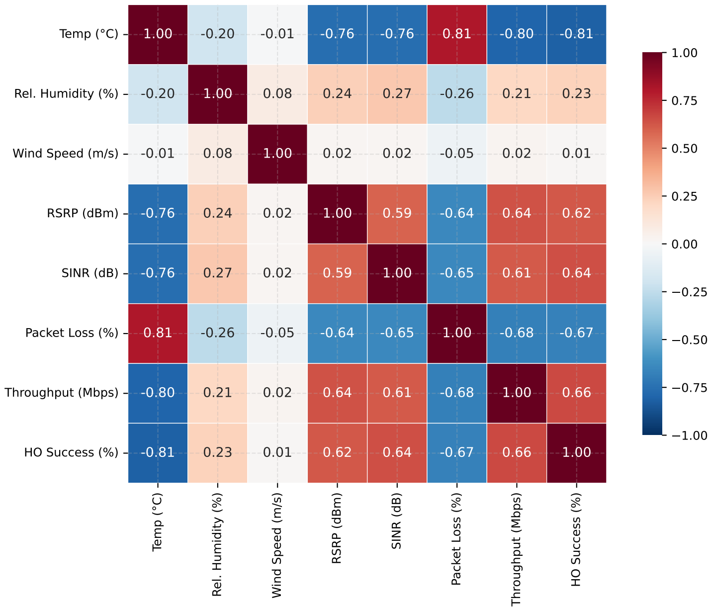
Figure 9 - Pearson Correlation Matrix Environmental Variables and Network KPIs
