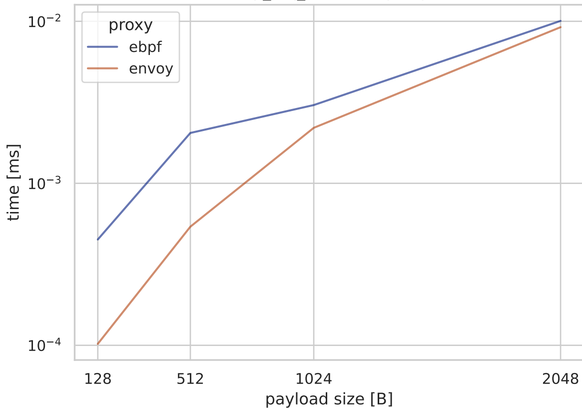
http_req_connecting avg
