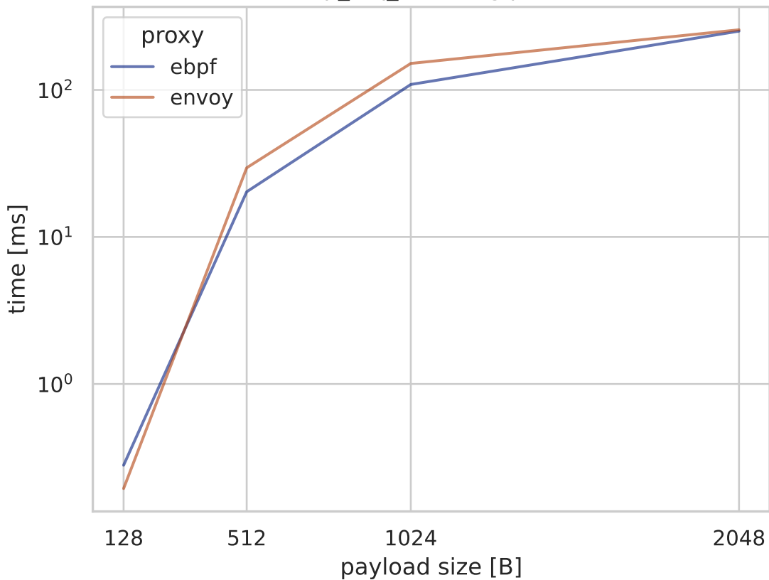
http_req_receiving p(95)
