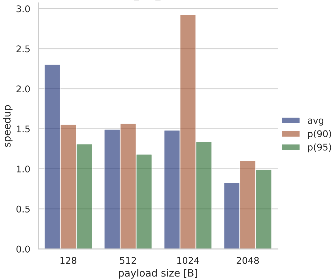
http_req_duration
