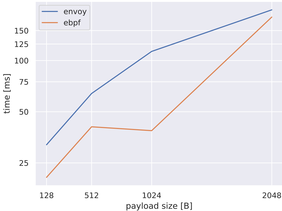
http_req_duration p(90)
