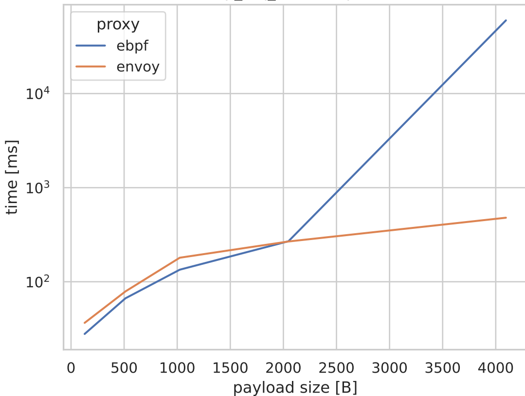
http_req_duration p(95)
