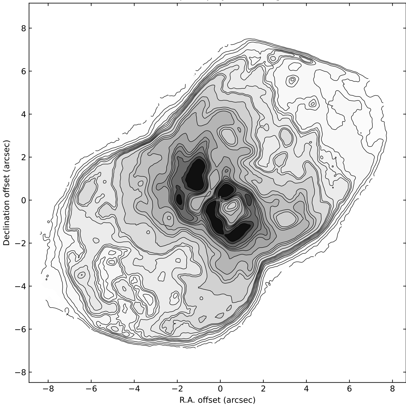
Reconstructed 18 um map (display smoothing 0.15 arcsec FWHM)
