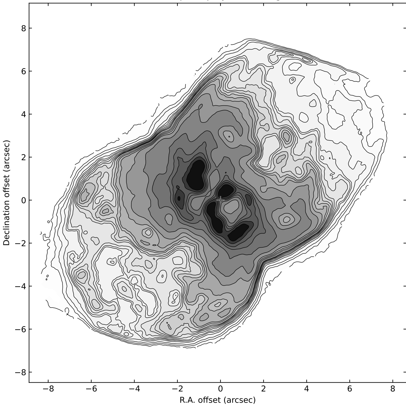
Reconstructed 18 \mu m map (display smoothing 0.15 arcsec FWHM)
