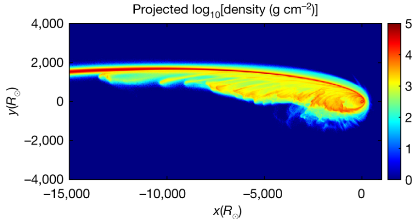
The projected log column density during a simulated tidal disruption event; positions are measured in solar radii. From E. Steinberg and N. C. Stone, “Stream–disk shocks as the origins of peak light in tidal disruption events,” Nature 625, 463–467 (2024), Fig. 1, doi:10.1038/s41586-023-06875-y.
