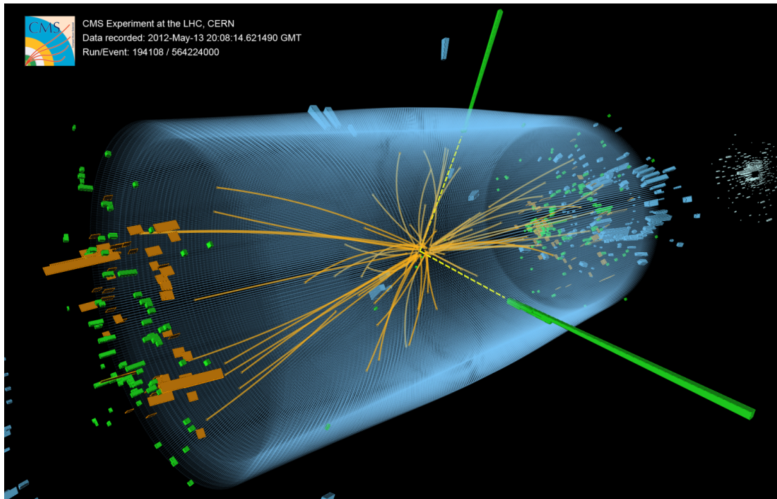
A CMS diphoton candidate from the Higgs search, drawn from reconstructed detector signals. Image: CMS/CERN, CERN Higgs boson overview.
