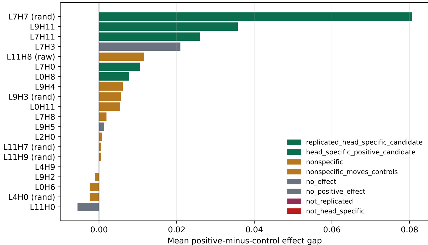
Head-specific causal gaps across seeds
